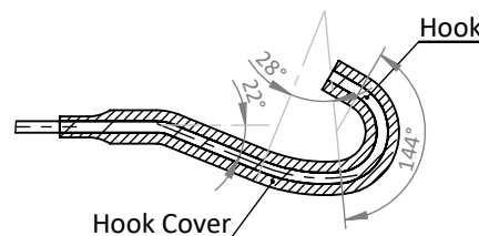
DETAIL J SCALE 1 : 2
